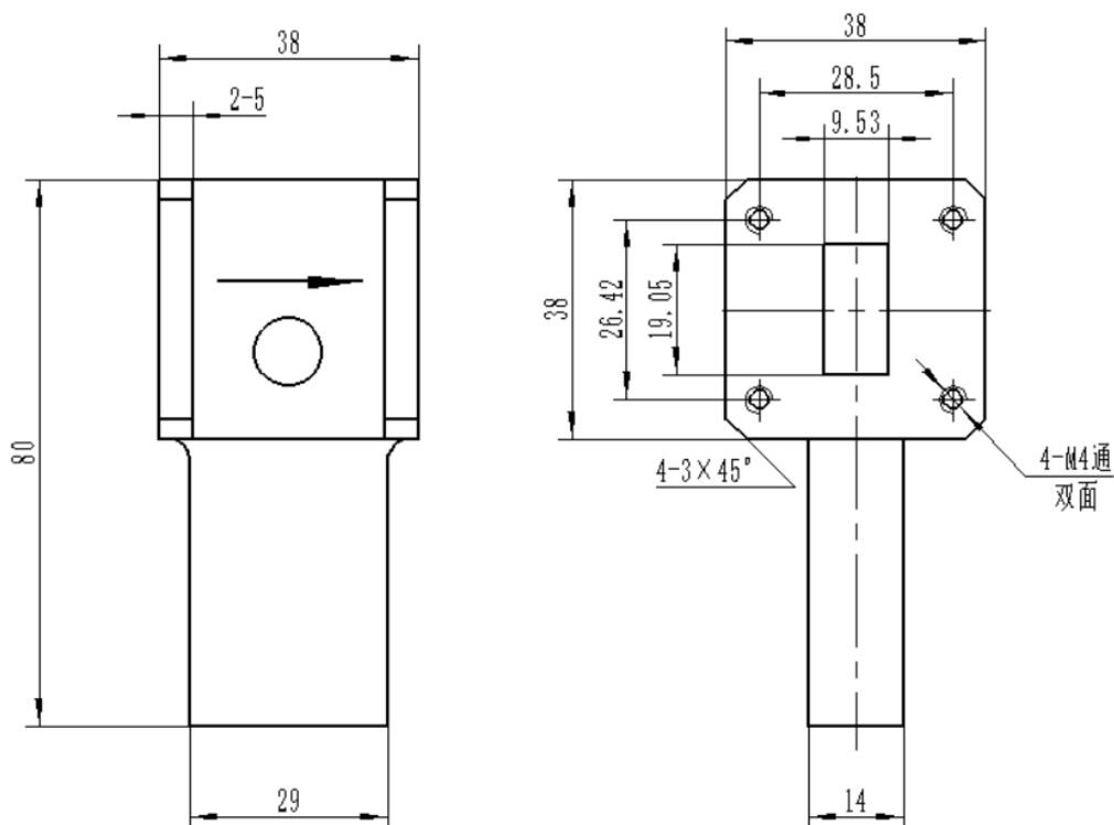
Mechanical Diagram (Unit: inch (mm))
