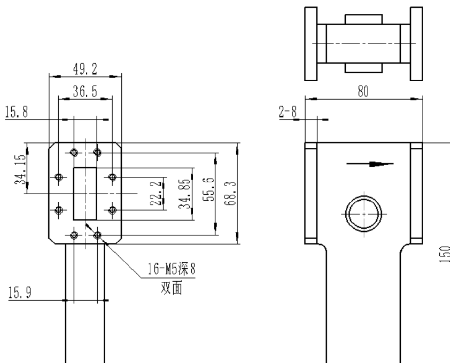
Mechanical Diagram (Unit: inch (mm))
