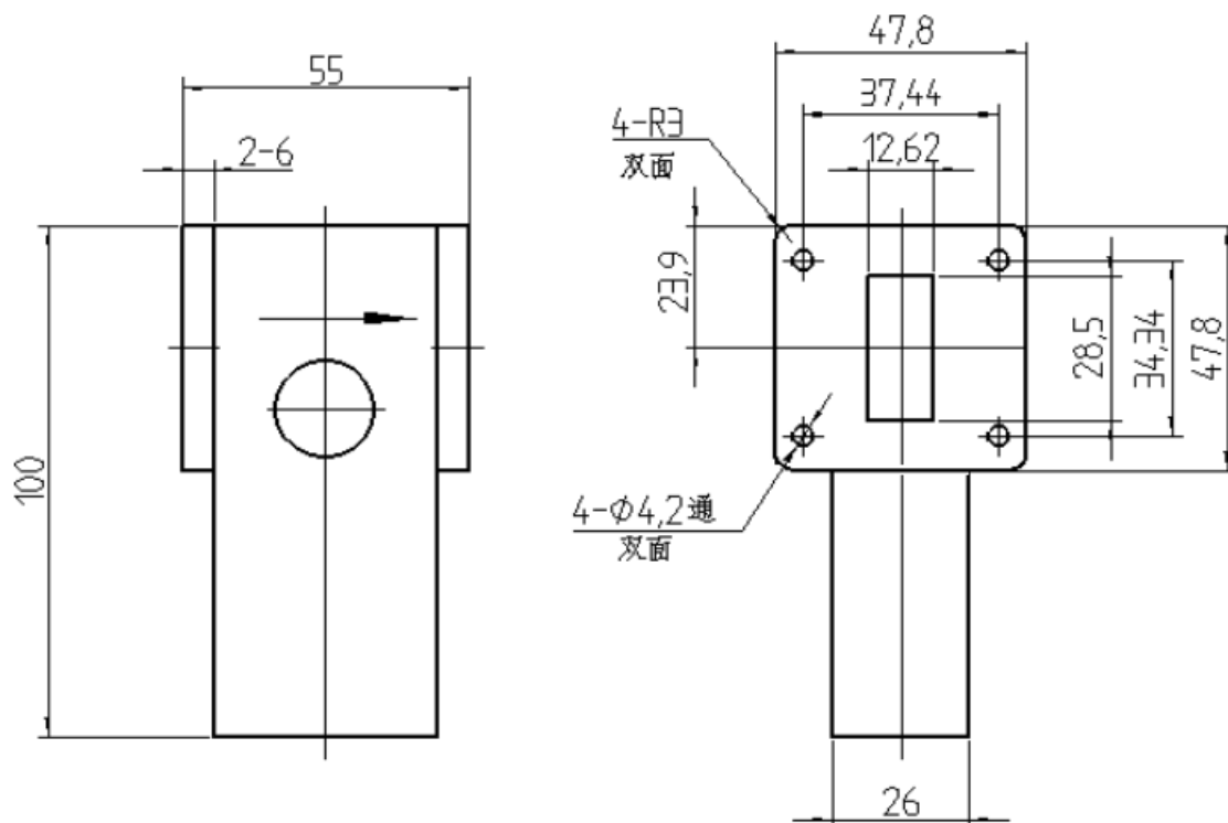
Mechanical Diagram (Unit: inch (mm))
